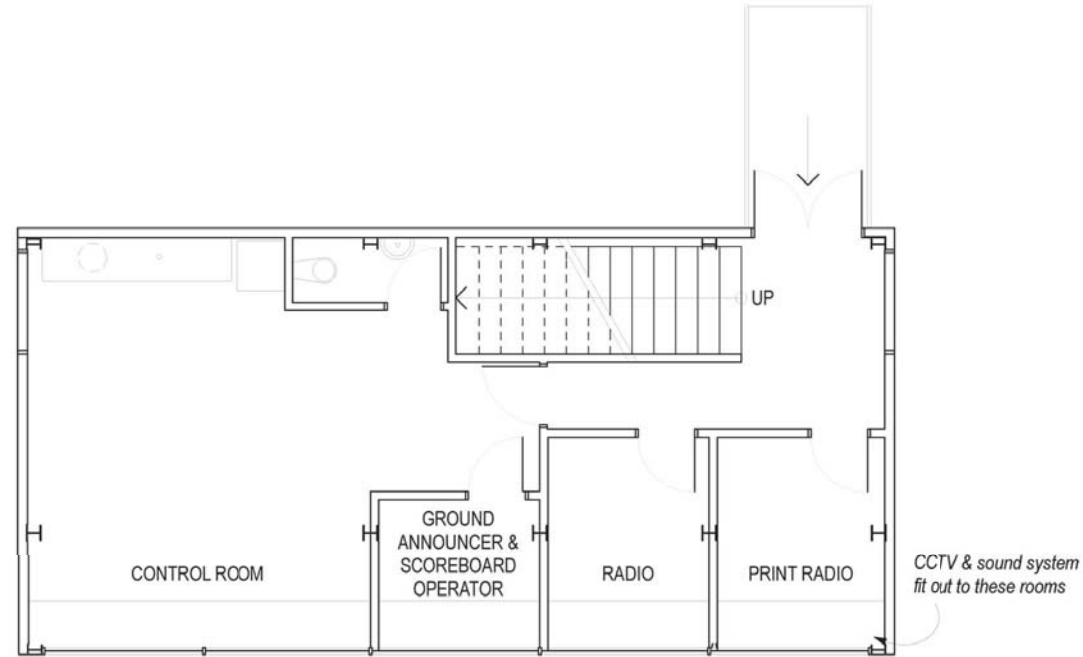
Media Centre Lvl 1 scale 1:100
