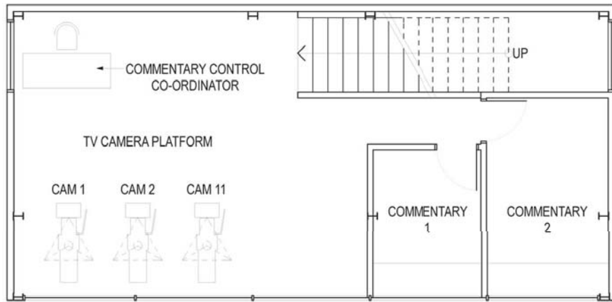
Media Centre Lvl 2 scale 1:100
