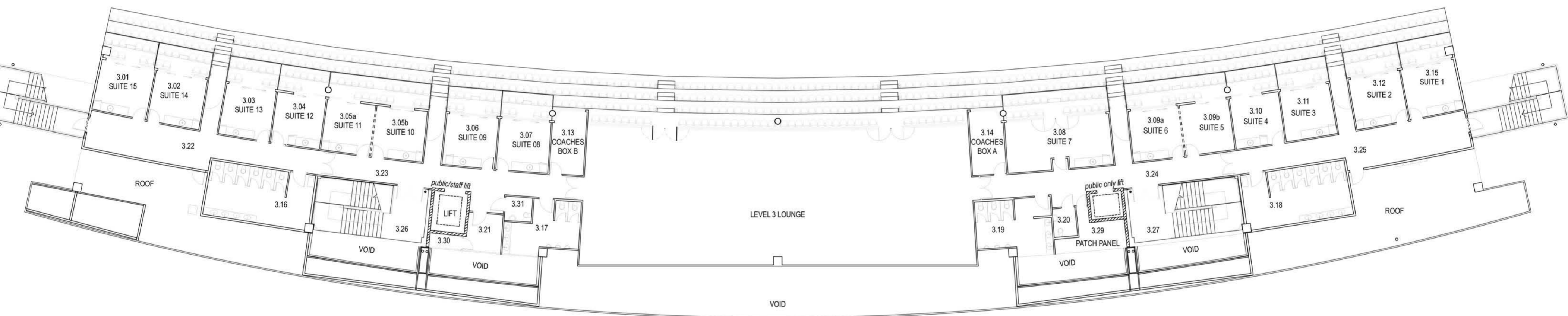
Level 3 scale 1:200
